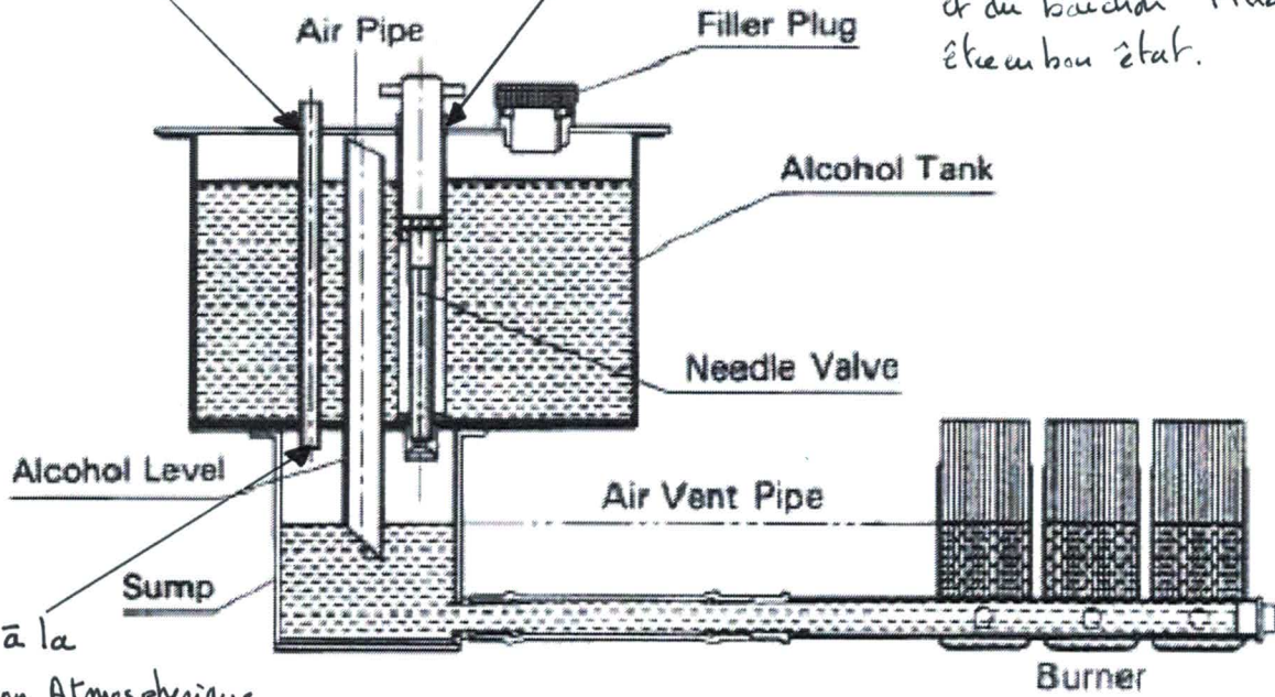
Fig.40 : Alcohol Tank and Burner
